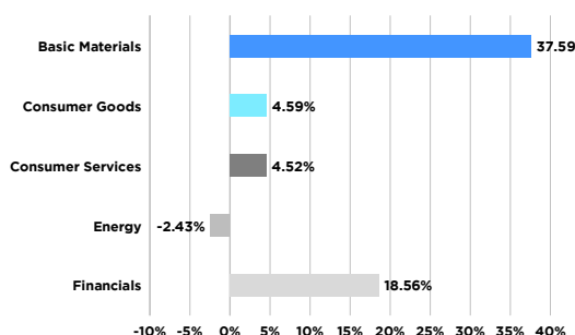
Exposure Statistics
