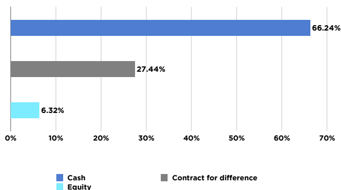
Exposure Statistics
